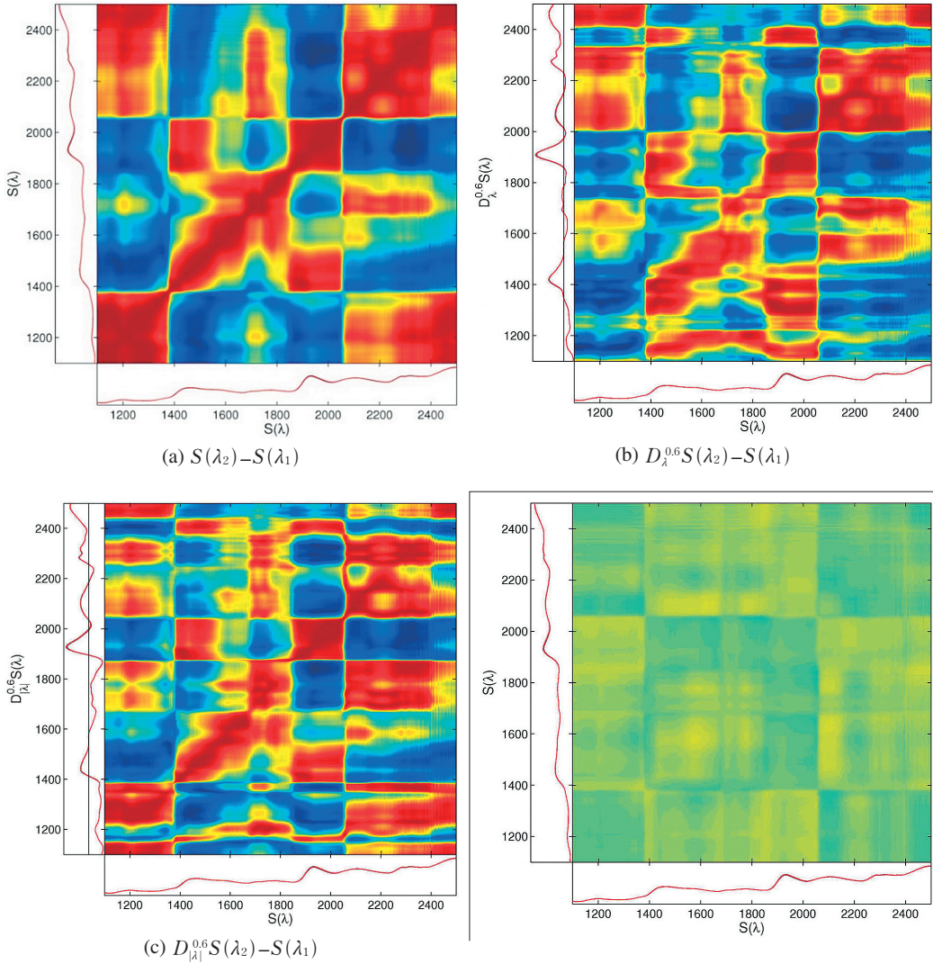
Fig. 2 Normalized 2D correlation spectra \rho(\lambda_1, \lambda_2) of the second order. Fig. 3 Normalized 2D correlation spectra \rho_3(\lambda_1, \lambda_2) : S(\lambda_2) - S(\lambda_1) of the third order.
